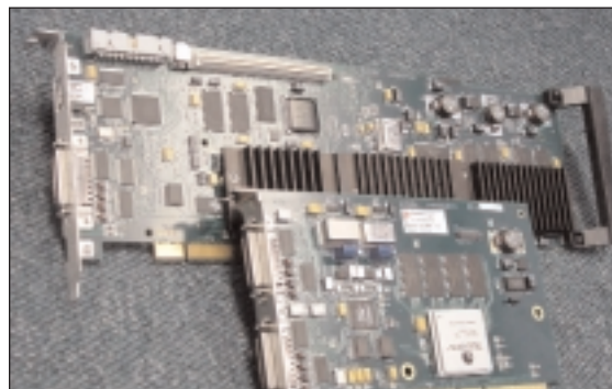
TARGA 3000 and TARGA Ciné With Digital Tether Ports on Left.
