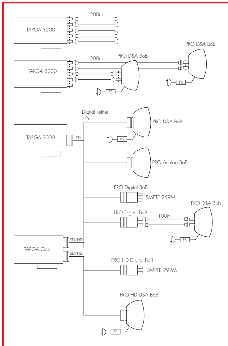
TARGA Connectivity Options.
