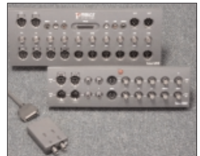
Digital Tether Break-Out boxes (BoB) for Audio and Video I/O.
